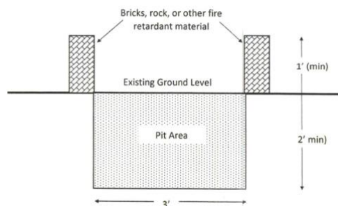
Example of Fire Pit Cross Section
